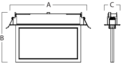
Semi-Recessed
